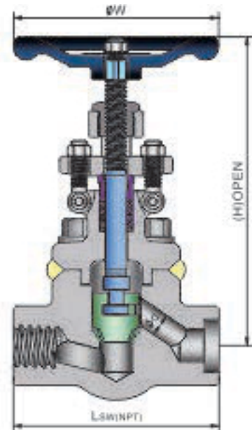
SW(NPT) WELDED BONNET 800,1500LB
