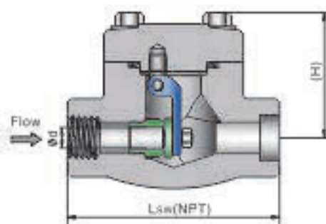
SWING TYPE, SW(NPT) BOLTED BONNET 800, 1500LB
