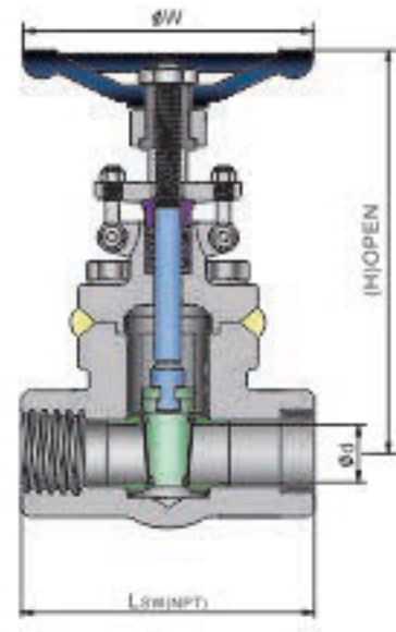
SW(NPT)WELDED BONNET 800,1500LB
