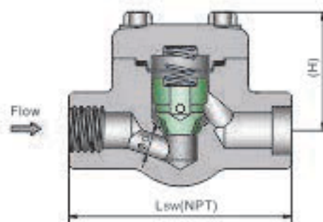
PISTON TYPE, SW(NPT) BOLTED BONNET 800, 1500LB
