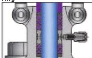
3.Grease injector & lantern ring
